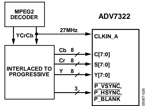
Figure 49. Progressive Scan Input Mode
