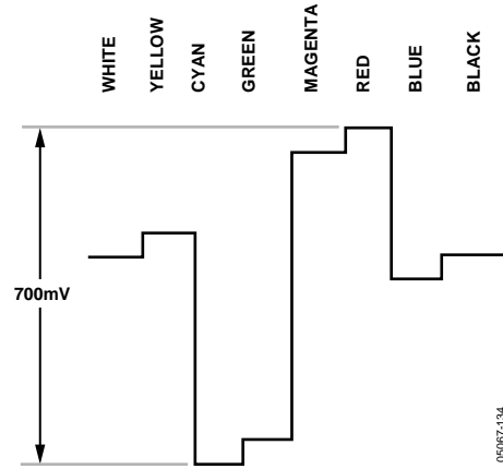
Figure 133. Pr Levels—PAL
