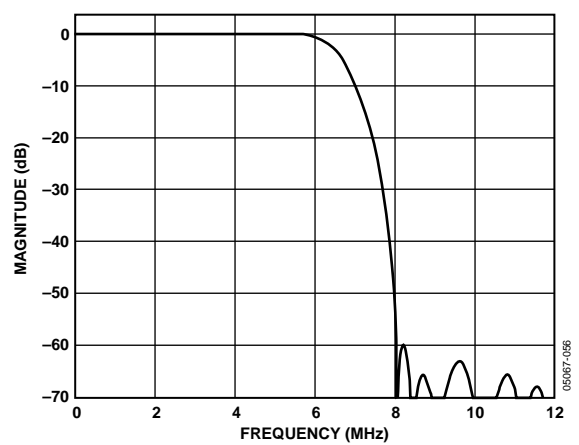
Figure 30. Y—16x Oversampling Filter
